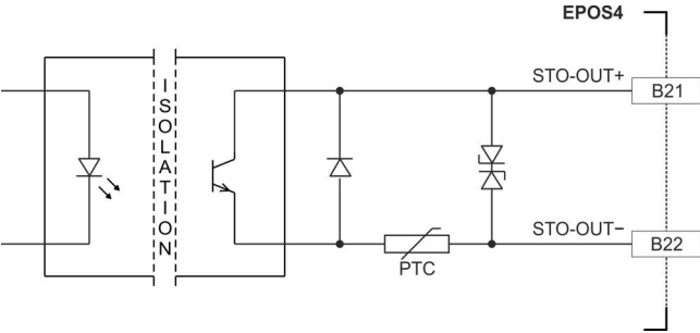
Figure 3-49 STO-OUT circuit
