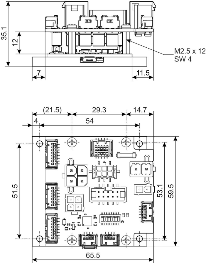
Figure 2-8 EPOS4 Compact 50/15 CAN – Dimensional drawing [mm]
