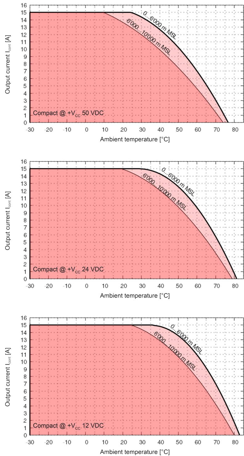
Figure 2-3 Derating of output current (operation without additional heat sink)
