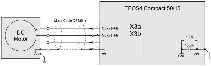
Figure 5-64 DC motor
