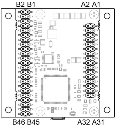
Figure 3-11 Pin assignment
