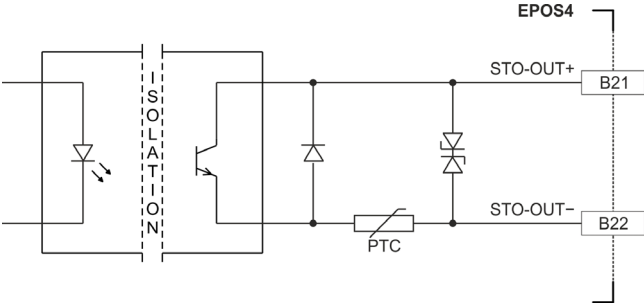
Figure 3-52 STO-OUT circuit
