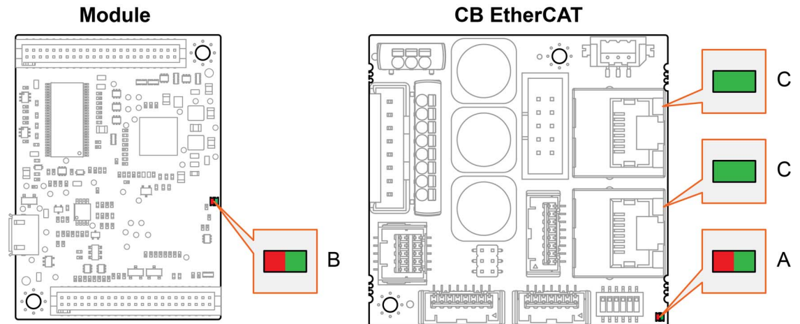
Figure 3-57 LEDs – Location
