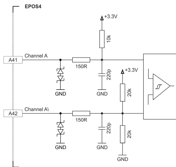
Figure 3-32 Encoder input circuit Ch A “differential” (analogously valid for Ch B &amp; Ch I)
