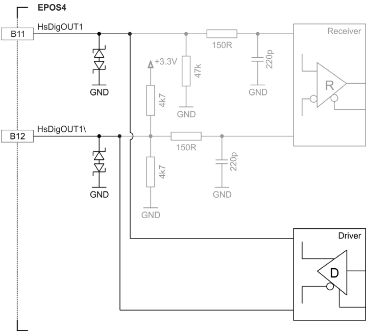
Figure 3-44 HsDigOUT1 output circuit
