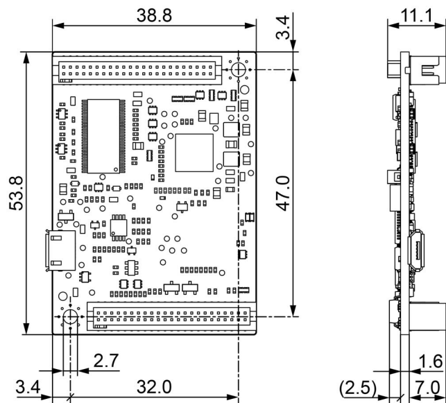
Figure 2-6 EPOS4 Module 24/1.5 – Dimensional drawing [mm]
