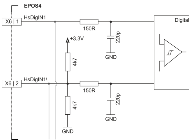
Figure 3-23 HsDigIN1 circuit “differential” (analogously valid for HsDigIN2...4)
